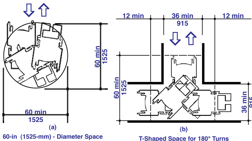
Fig. 3 Wheelchair Turning Space
